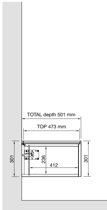
Storage unit with flap door
