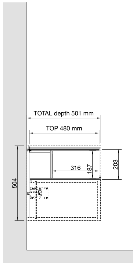
Open compartment on storage units with flap door
