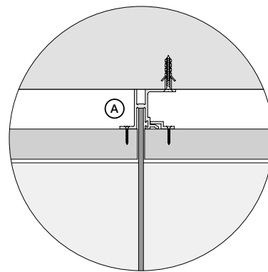
A = High central racks
