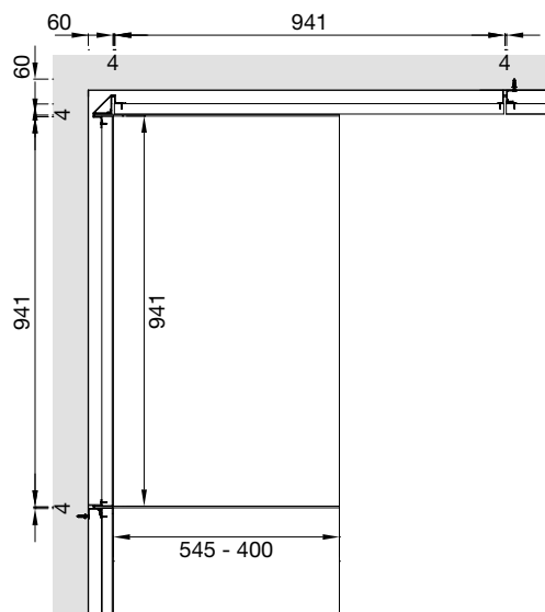
standard corner back panel equipped with standard shelf width 941
