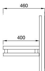
walk-in closet Ubik d 460 standard
