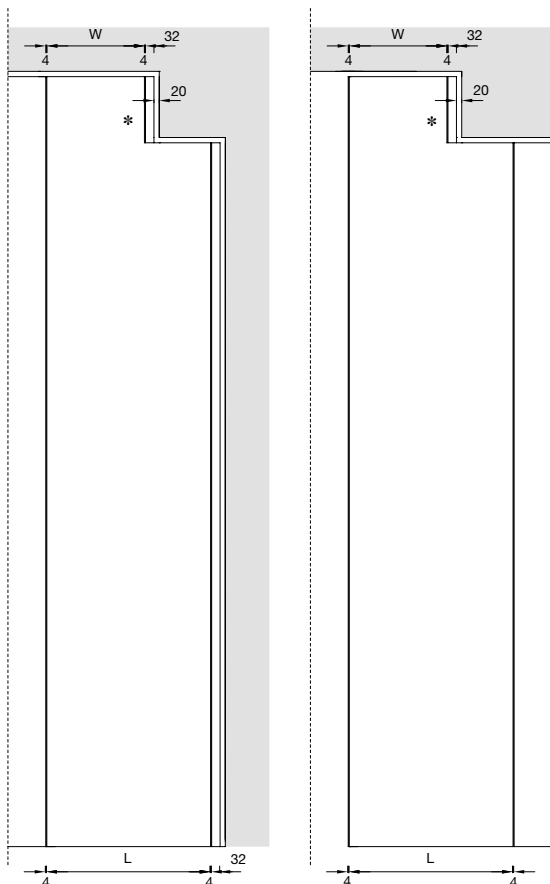
Back panel with shaping upper shaping
