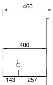
walk-in closet Ubik d 460 standard
