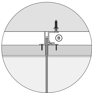
B = Low central racks
