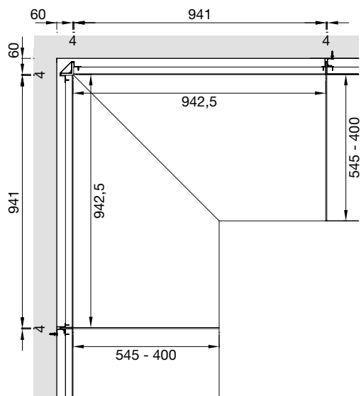
standard corner back panel equipped with standard corner shelf
