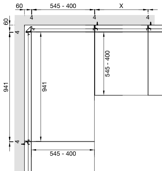
corner back panel with 1 customized side equipped with standard shelf width 941
