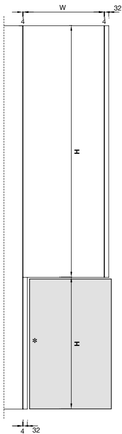
Back panel with shaping upper shaping
