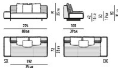
SPRING ELEMENTO TERMINALE HIGH SQUARE CM 225 SPRING ELEMENT WITH 1 ARMREST HIGH SQUARE CM 225
