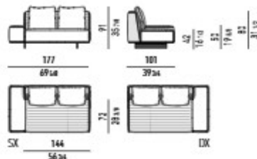
SPRING ELEMENTO TERMINALE HIGH SQUARE CM 177 SPRING ELEMENT WITH 1 ARMREST HIGH SQUARE CM 177
