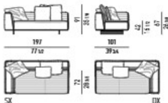
SPRING ELEMENTO TERMINALE LOW CM 197 SPRING ELEMENT WITH 1 ARMREST LOW CM 197
