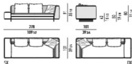
SUITE DIVANO HIGH SQUARE MIX CM 278 SUITE SOFA HIGH SQUARE MIX CM 278
