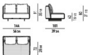
SPRING ELEMENTO CENTRALE HIGH CM 144 SPRING CENTRAL ELEMENT HIGH CM 144
