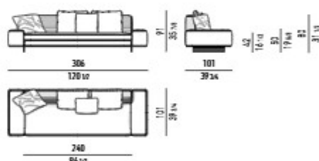
SUITE DIVANO HIGH SQUARE CM 306 SUITE SOFA HIGH SQUARE CM 306
