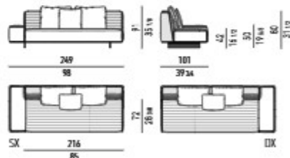
SPRING ELEMENTO TERMINALE HIGH SQUARE CM 249 SPRING ELEMENT WITH 1 ARMREST HIGH SQUARE CM 249
