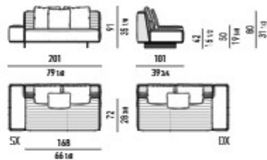
SPRING ELEMENTO TERMINALE HIGH SQUARE CM 201 SPRING ELEMENT WITH 1 ARMREST HIGH SQUARE CM 201
