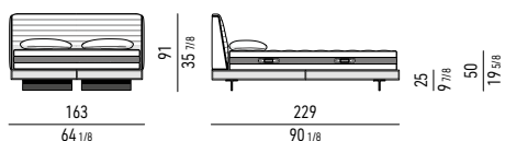
LETTO QUEEN SIZE CM 163X229 BED QUEEN SIZE CM 163X229
