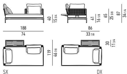
TEAK ELEMENTO TERMINALE DAYBED CON TOP CM 188X119 TEAK DAYBED ELEMENT WITH 1 ARMREST WITH TOP CM 188X119
