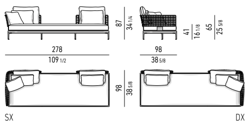
TEAK ELEMENTO TERMINALE OPEN CM 278X98 TEAK OPEN ELEMENT WITH 1 ARMREST CM 278X98
