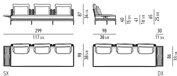
TEAK ELEMENTO TERMINALE CON TOP CM 299X98 TEAK ELEMENT WITH 1 ARMREST WITH TOP CM 299X98
