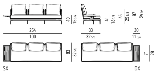
TEAK ELEMENTO TERMINALE CON TOP CM 254X83 TEAK ELEMENT WITH 1 ARMREST WITH TOP CM 254X83
