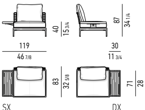
TEAK LOVESEAT SENZA BRACCIOLI CON TOP CM 119X83 TEAK LOVESEAT WITHOUT ARMRESTS WITH TOP CM 119X83
