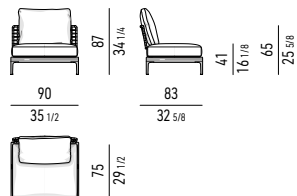
TEAK LOVESEAT SENZA BRACCIOLI CM 90X83 TEAK LOVESEAT WITHOUT ARMRESTS CM 90X83
