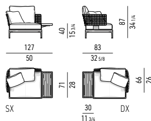
TEAK LOVESEAT CON TOP CM 127X83 TEAK LOVESEAT WITH TOP CM 127X83
